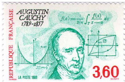
Theory of Equations. Augustin-Louis Cauchy (1789-1857). http://www.1902encyclopedia.com/A/ALG/algebra-14.html
