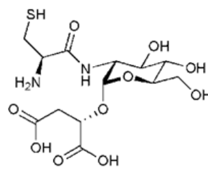
Bacillithiol
