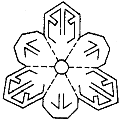
FIGURE 1.2 The symmetry content of several patterns.
